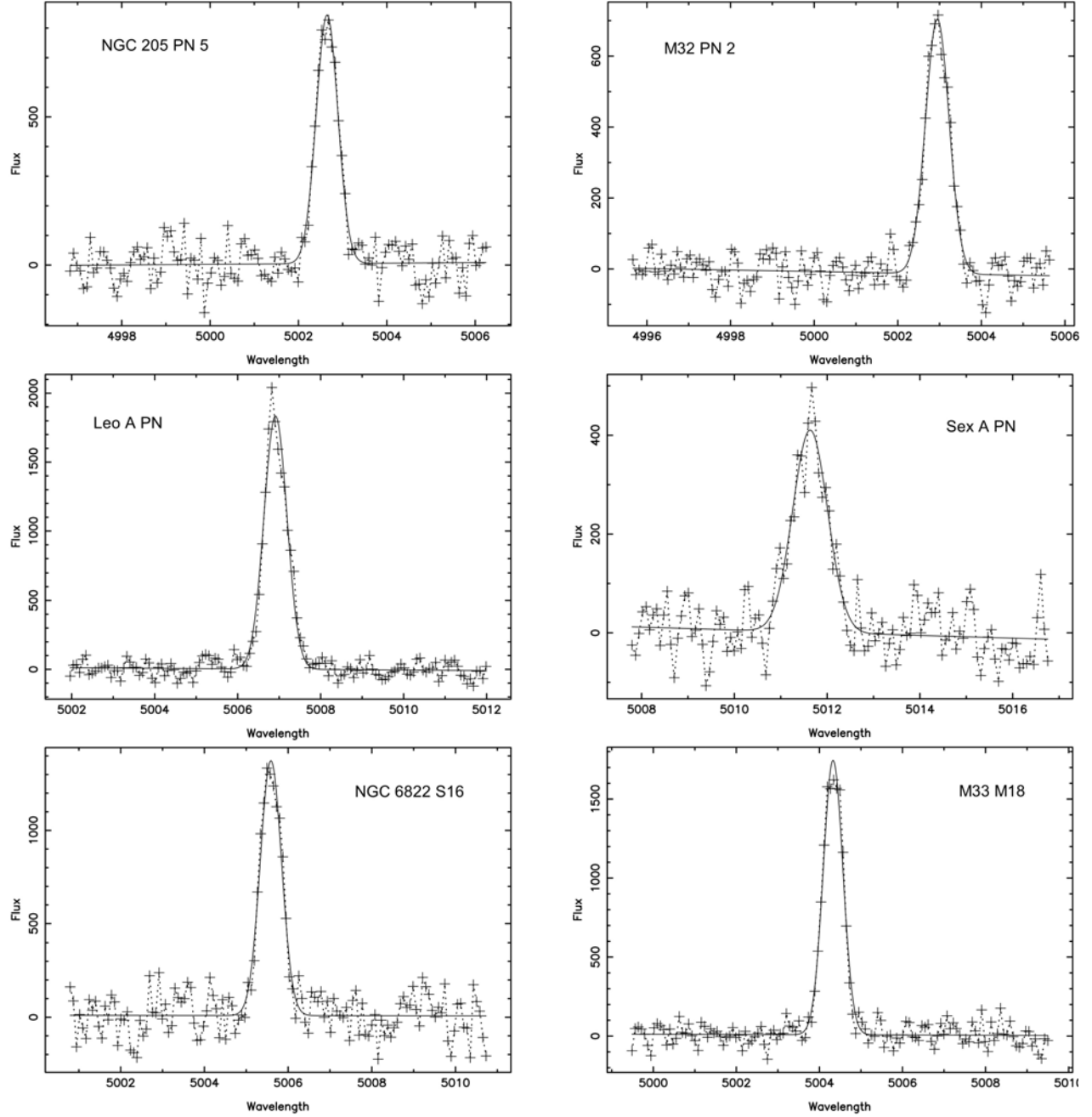
Fig. 3. The line profiles are shown for planetary nebulae in NGC 205, M32, the dwarf irregular galaxies Leo A, Sex A, and NGC 6822, and the spiral galaxy M33. Deviations of the data about the Gaussian fit are insignificant, even though these are among the profiles with the best S/N in these galaxies. See Figure 2 for further details.
