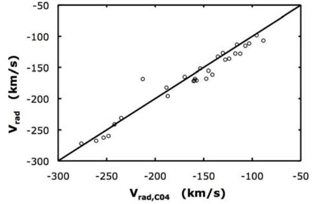
Fig. 7. We compare our radial velocities with those measured by Ciardullo et al. (2004) for planetary nebulae in M33. The solid line indicates the locus of identical radial velocities. Our velocities are offset, by -13.8\text{ km s}^{-1} .
