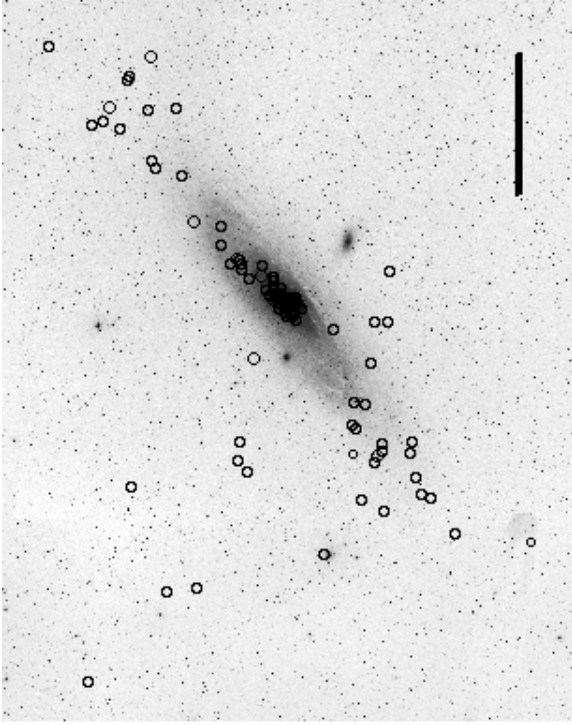
Fig. 9. The planetary nebulae observed in M31 are shown overplotted on a DSS image of M31, M32, and NGC 205. The bar is one degree in length. North is up and east is to the left.
