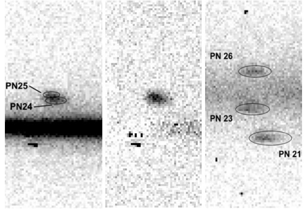
Fig. 1. The left panel presents the raw two-dimensional spectrum for PN24 and PN25 in M32 (east is up, bluer wavelengths to the left). The continuous emission below them (to the west) is from M32's nuclear region. The planetary nebulae are sufficiently close together that their emission is merged into a single teardrop-shaped profile. The middle panel presents the same spectrum for PN24 and PN25 once M32's continuous emission had been filtered out. For comparison, the right panel presents the two-dimensional spectrum for PN26, PN23, and PN21 in M32 (ordered north to south; north is up, bluer wavelengths to the left) at the same spatial scale and taken immediately prior to the spectrum of PN24 and PN25 (continuous emission from M32 is again visible). The two-dimensional (spatially-merged) spectrum of PN24 and PN25 is clearly more complex than the spectra of PN26, PN23, or PN21. PN25 is to the east (above) of PN24, has a more blueshifted radial velocity, and a narrower line profile (see Table 2), the two effects explaining the tilted teardrop shape of the combined profile. The "individual" profiles for PN24 and PN25 were obtained by splitting the combined emission at the spatial centre.
