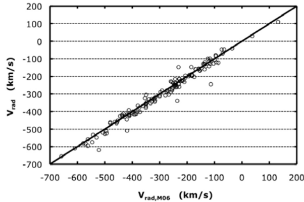
Fig. 6. We compare our radial velocities with those measured by Merrett et al. (2006, M06) for planetary nebulae in M31, M32, and NGC 205. The solid line indicates the locus of identical radial velocities. Our velocities are offset slightly, by -3.3\text{ km s}^{-1} .
