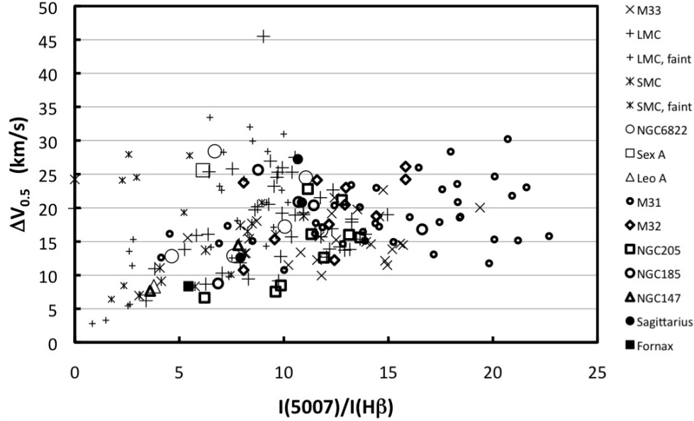
Fig. 13. We plot the [\text{O III}]\lambda 5007 line width as a function of the I(5007)/I(\text{H}\beta) ratio for the planetary nebulae with low resolution spectra (see the literature cited in Figure 11). The symbols follow the same scheme as in Figure 11. Here, most of the M31 planetary nebulae are from its bulge. In part, the higher oxygen abundances for the planetary nebulae in M31's bulge allow them to achieve higher I(5007)/I(\text{H}\beta) ratios than those for planetary nebulae elsewhere. However, the planetary nebulae in M32 and the dwarf spheroidals tend to have systematically larger ratios than their counterparts in the dwarf irregulars, even though they have similar oxygen abundances, so nebular structure or the distribution of central star temperatures also likely play a role in elevating the I(5007)/I(\text{H}\beta) ratios for planetary nebulae in systems without star formation.
