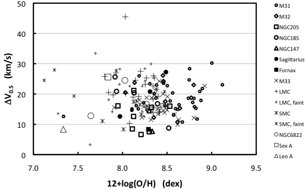
Fig. 11. We plot the [\text{O III}]\lambda 5007 line width as a function of the oxygen abundance for the planetary nebulae with low resolution spectra. The symbols for galaxies without star formation are in bold or filled while the symbols for galaxies with ongoing star formation are light and unfilled. Bright and faint planetary nebulae in the Magellanic Clouds are distinguished by large and small symbols, respectively. For M31, the planetary nebulae come overwhelmingly from the bulge. Galactic systems with and without star formation cover the abundance range from 7.9 < 12 + \log(\text{O}/\text{H}) < 8.5 , but planetary nebulae from the bulge of M31 dominate higher abundances. There is no strong variation in line width with abundance or between galactic systems with and without star formation. The oxygen abundances are taken from Richer & McCall (2008) and Magrini, Stanghellini, & Villaver (2009); the former adopting data from Jacoby & Ford (1986), Aller et al. (1987), Barlow (1987), Monk, Barlow, & Clegg (1988), Wood et al. (1987), Dopita et al. (1988), Meatheringham, Dopita, & Morgan (1988), Henry, Liebert, & Boroson (1989), Meatheringham & Dopita (1991a,b), Dopita & Meatheringham (1991), Vassiliadis et al. (1992), Jacoby & Kaler (1993), Leisy & Dennefeld (1996), Walsh et al. (1997), Jacoby & Ciardullo (1999), Richer, Stasińska, & McCall (1999), Roth et al. (2004), Kniazev et al. (2005), Magrini et al. (2005), van Zee, Skillman, & Haynes (2006), Zijlstra et al. (2006), Gonçalves et al. (2007), Kniazev et al. (2007), and Richer & McCall (2007, 2008).
