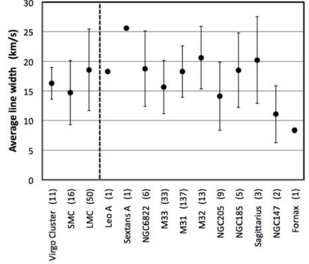
Fig. 8. We compare the average [\text{O III}]\lambda 5007 line width from Table 2, \Delta V_{0.5} , found for the planetary nebulae in different galaxies. The “error bars” indicate the standard deviations of the line width distributions. The number in parentheses indicates the number of planetary nebulae observed in each galaxy. Clearly, the average line width does not vary much among different galaxies. The data for the Magellanic Clouds are taken from Dopita et al. (1985, 1988) for planetary nebulae within 2.5 \text{ mag} of the PNLf peak. The data for the Virgo Cluster are taken from Arnaboldi et al. (2008).
